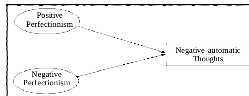
Fig. 1: Research model
