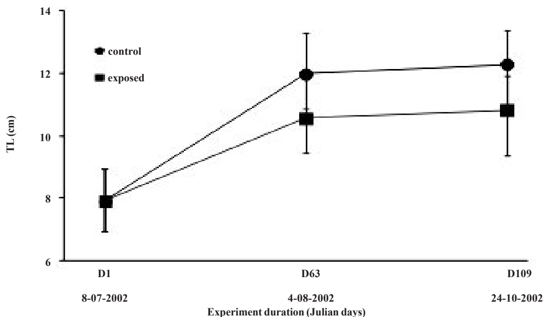
Fig 1. Evolution of total length TL (cm) (mean ± standard deviation) in control and exposed 0-group sole juveniles during the monitoring phase in mesocosm
