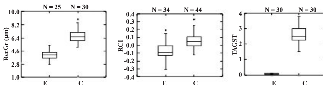
Fig. 2. Biological indicators (median, \pm SD; 95% confident interval and outliers) measured in control (C) and exposed (E) 0-group sole juveniles. RecGr ( \mu\text{m} ): Recent Growth; RCI (mg): morphometric condition; TAG:ST : triacylglycerol to free sterol ratio; n: number of individuals
