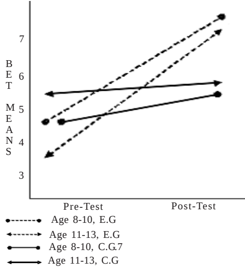
Fig. 1. BET by age interaction
