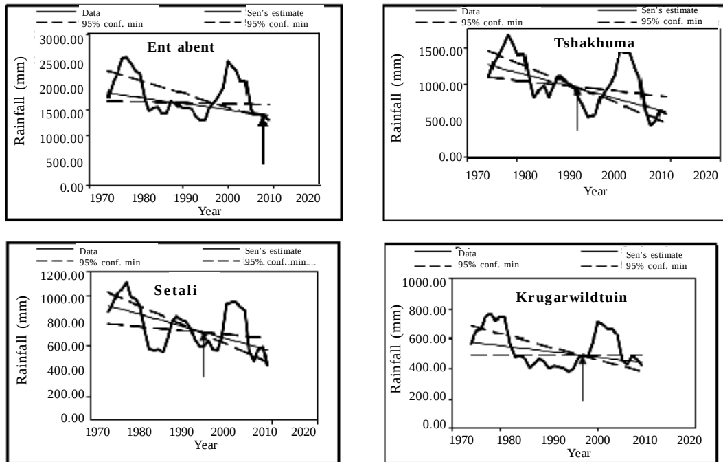
Fig. 2. Humid-Zone rainfall trend; the arrow indicates the position where the trend show high level of significance ( \geq 95\% )
