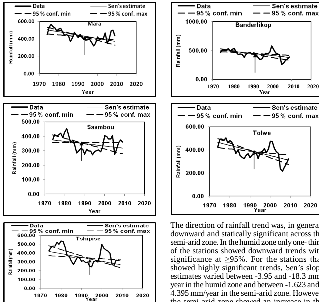
Fig. 3. Semi-arid-zone rainfall trend analysis; the arrow indicates the position where the trend shows high level of significance ( \geq 95\% ).
