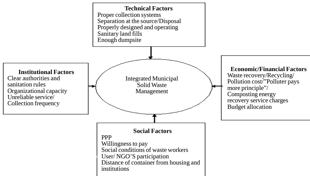
Fig. 1. Conceptual framework
