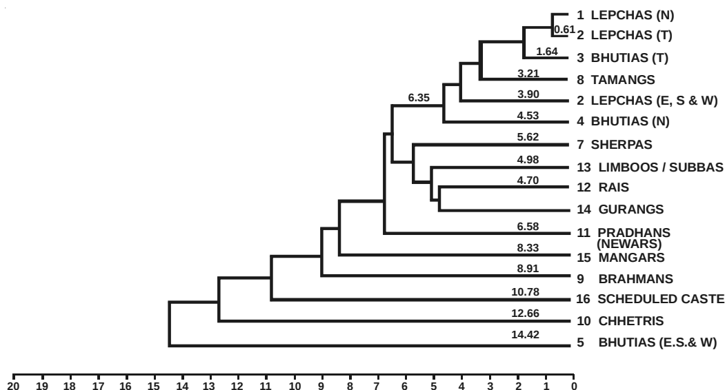
Fig. 3. Dendrogram of the various population groups of Sikkim.
