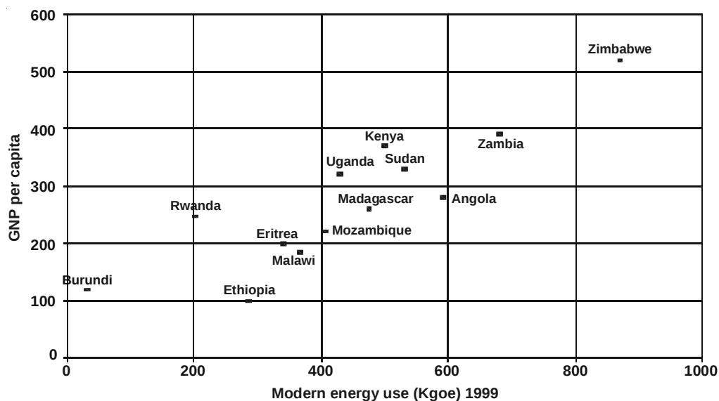
Fig. 3. Relationship between national income and energy
