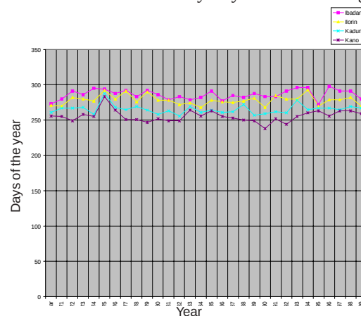
Fig. 9. Rainfall retreat dates, using rainy days (1961-2000)
