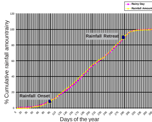
Fig. 2. Mean rainfall onset and retreat dates in Ibadan (1961-2000).
