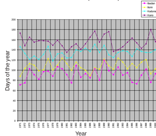
Fig. 8. Rainfall onset dates, using rainy days (1971-2000)
