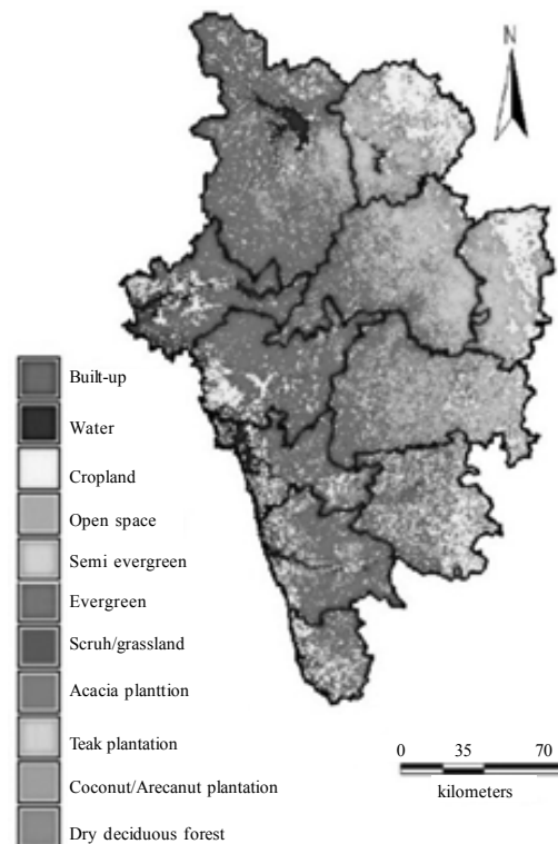
Fig. 3. Land-use classification map of Uttara Kannada district
