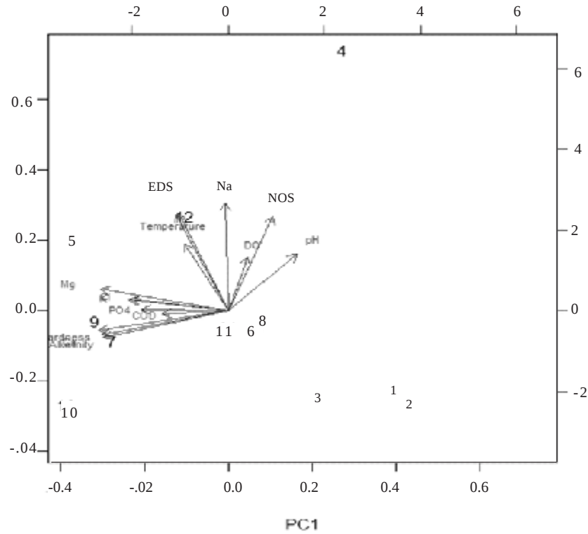
Fig. 4. Loadings of the 15 experimental variables and scores of the lakes (1-12) on the plane defined by principal components 1 and 2
