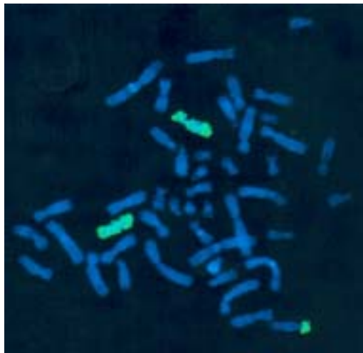
Fig.5. Metaphase after FISH with wcp 12, both normal chromosomes 12 and the additional segment on the short arm of chromosome 14 show hybridisation signals.
