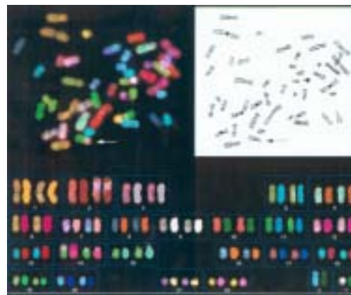
Fig. 4. Metaphase spread after simultaneous SKY-hybridisation of 24 combinatorially labelled chromosome-painting probes. Chromosomes are shown in RGB display colours (A); chromosome spectra are visualised by applying an RGB look up table to different regions of the spectrum, for each homologue chromosome it is shown on the left side the display colour and of the identical chromosome on the right side the spectra based colour (B); electronically inverted DAPI image (C); the aberrant chromosome 14 is denoted by arrow.
