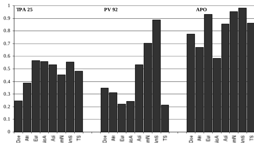
Fig 2. World distribution of the weighted mean frequencies of the Alu insertions TPA 25, PV 92 and APO (Batzner et al., 1996; Batzner et al., 1991; Batzner et al., 1994; Comas et al., 2000; Melton et al., 1998; Novick et al., 1998; Novick et al., 1995; Parra et al., 2001; Parra et al., 1998; Perna et al., 1992; Stepanov et al., 1999; Stoneking et al., 1997; Tishkoff et al., 1996; van der Bom et al., 1997; Watkins et al., 2001). Oce: Oceania; Afr: Africa; Eur: Europe; NoA: North America; Asi: Asia; AmN: Amerindians-North America; AmS: Amerindians-South America; TS: This Study.
