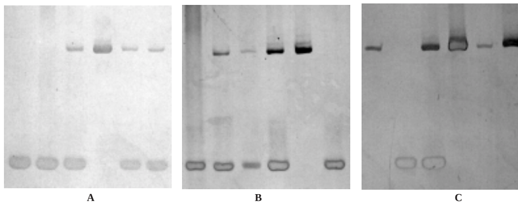
Fig. 1. PAGE, 6% non-denaturing, stained with silver nitrate. A. Locus TPA 25; B. Locus PV92; C. Locus APO. In the LANE A4, B5, C1, C4, C5 and C6, ii homozygous; in the LANE A3, A5, A6, B2, B3, B4 and C3, heterozygous and in the LANE A1, A2, B1, B6 and C2, homozygous aa .
