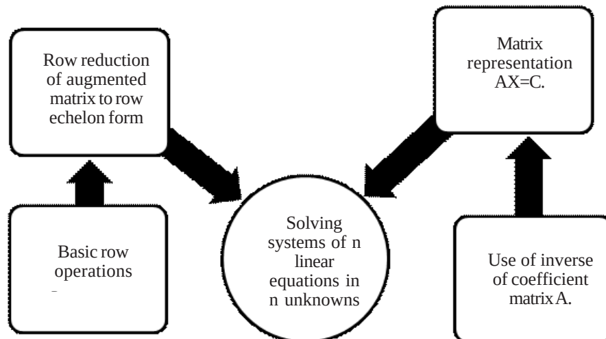
Fig.1. A schema to solve a system of n linear equations in n unknowns Source: Author
