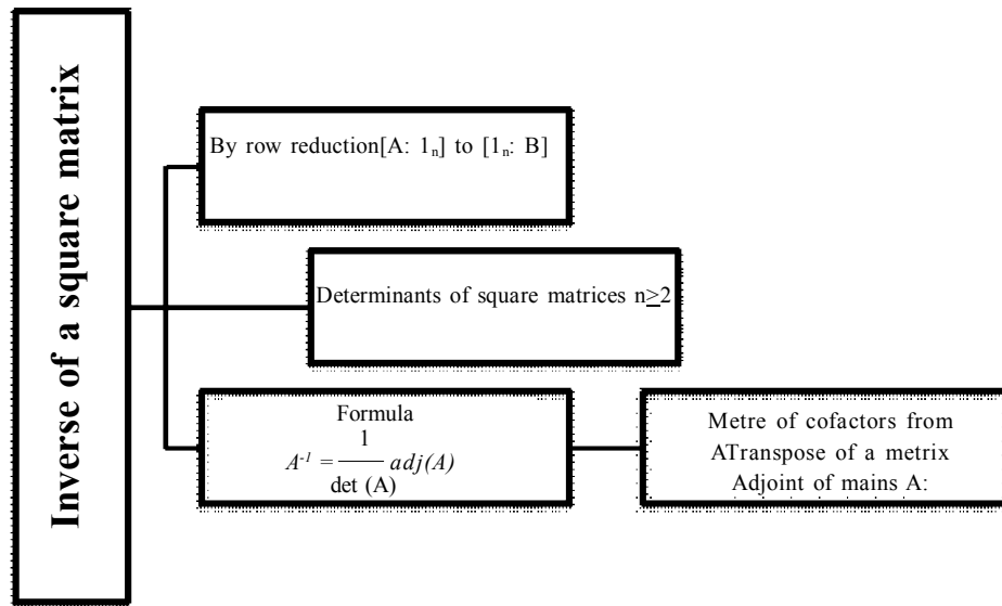
Fig. 2. Schema for inverse of a matrix Source: Author
