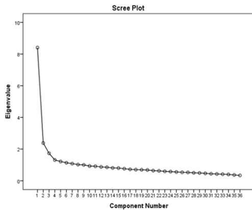
Fig. 1. The scree plot graph of the scale
